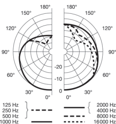
Polar Pattern
