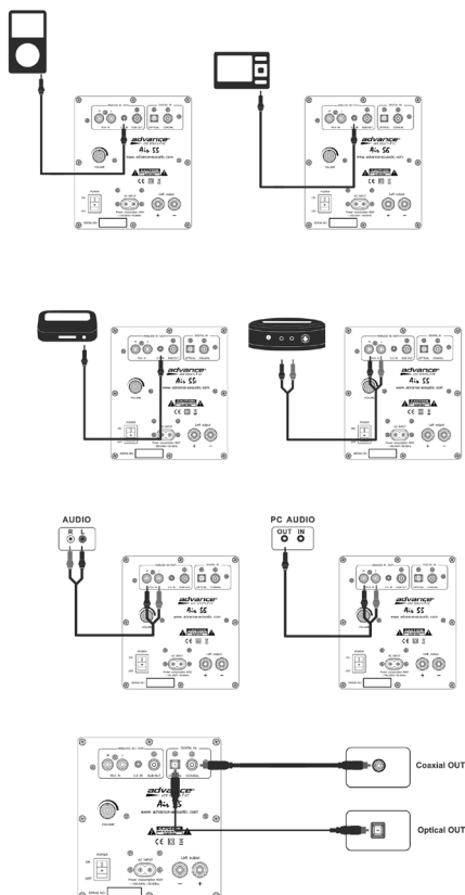
General connections
