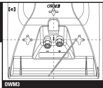
FIGURE 5c ANGLED/CORNER WALL MOUNT TEMPLATE
