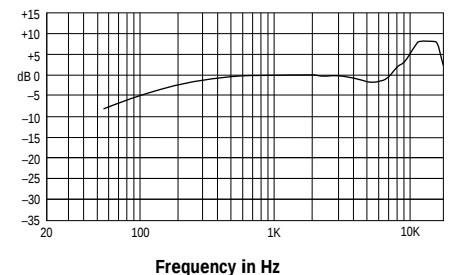
Fig. 1 Frequency Response
