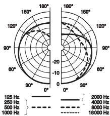
Diagrama polar (hipercardioide)
