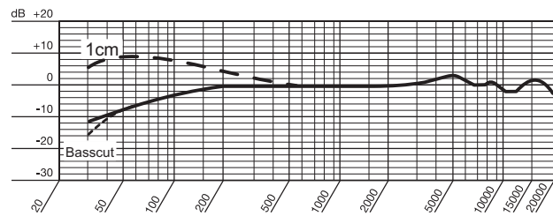
Frequenzgang (Hyperniere)
